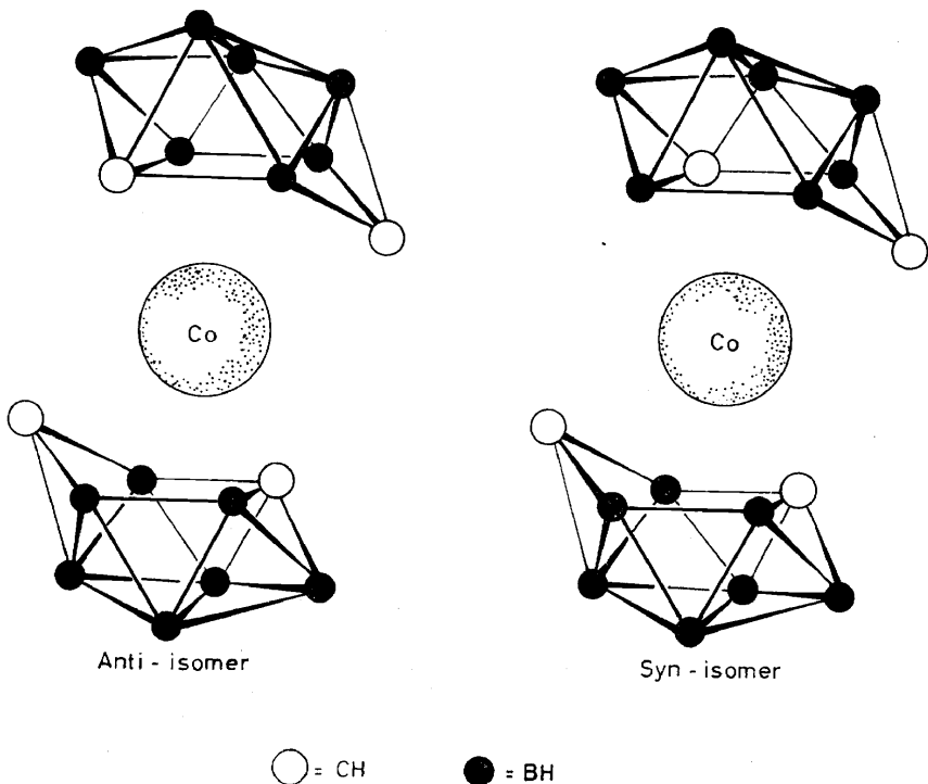
Figure 13. Simplified structures of isomeric [\pi\text{-B}_7\text{C}_2\text{H}_5]_2\text{Co}^- ions. Actual structure was shown to be that of the anti-isomer
