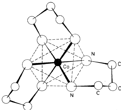
Figure 10. A drawing of the complex ion (-)\text{D-}[\text{Co}(\text{tn})_3]^{3+} .
