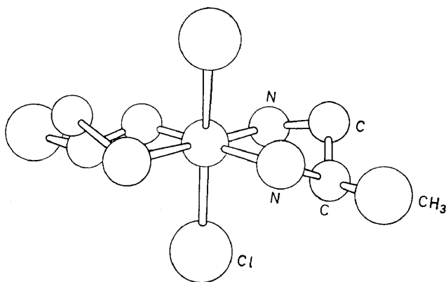
Figure 3. A perspective drawing of the complex ion (-)\text{-D-[CoCl}_2(\text{l-pn})_2]^+
