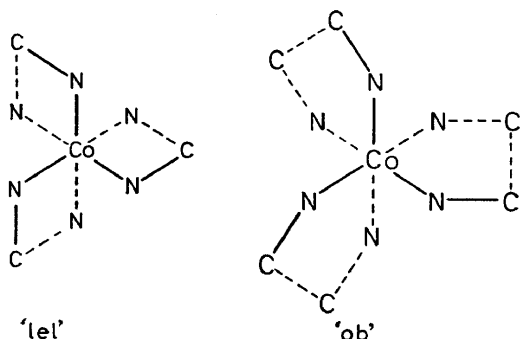
Figure 5. The 'lel' and 'ob' forms of the complex ion [\text{Co}(\text{en})_3]^{3+} .
