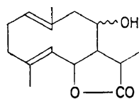
Isobalchanolide
