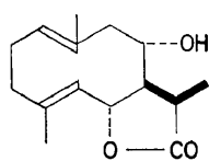
Balchanolide
