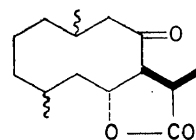
Arctiopicrin Cnicin
