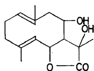
11-Hydroxybalchanolide
