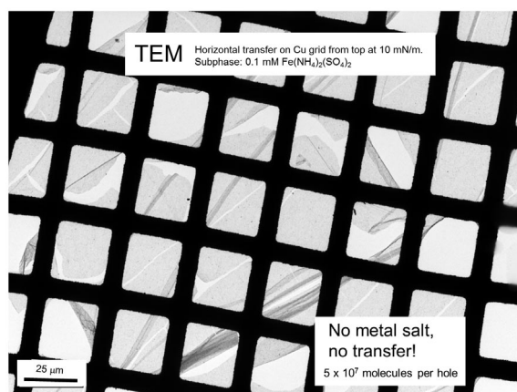
Fig. 3 TEM micrograph of a film of monomer M6 horizontally transferred from the air/water interface after exposing it to 0.1 mM \text{Fe}(\text{NH}_4)_2(\text{SO}_4)_2 from the subphase. Reproduced with permission from ref. [21].
