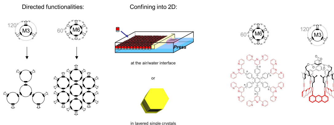
Fig. 1 Left: Two strategies that could eventually lead to 2D polymers and concrete molecular structures of monomers used for both strategies; right: the hexa-terpyridine M6 for the interfacial approach and the cyclic tris-anthracene M3 for the single-crystal approach.
