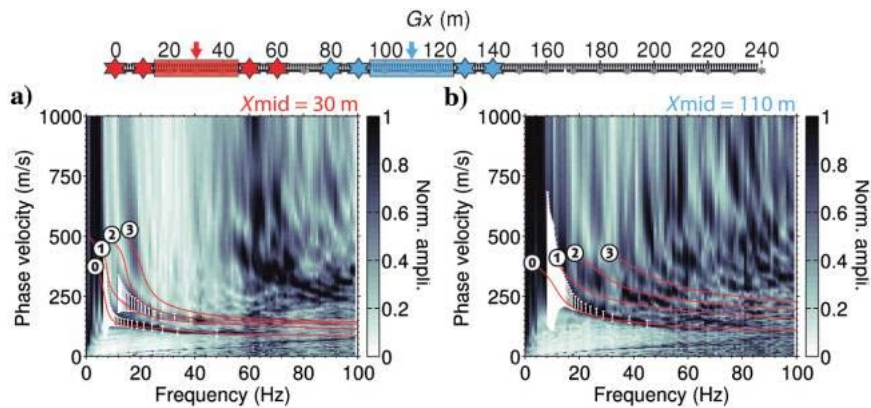
Figure 6.12 Stacked dispersion images extracted at (a) X_{mid} = 30 m and (b) X_{mid} = 110 m with picked (white error bars) and calculated (solid red lines) dispersion curves represented for the fundamental (0), the first (1), second (2), and third (3) higher modes. From Pasquet and Bodet (2017).
